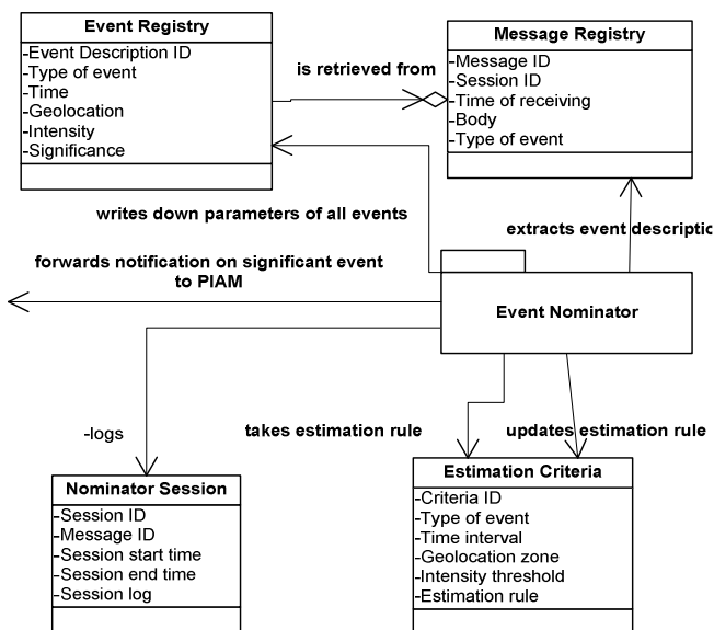
Fig. 3. Event Nominator data model.
