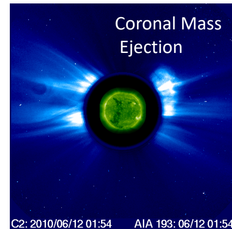
SOHO/SDO Image
