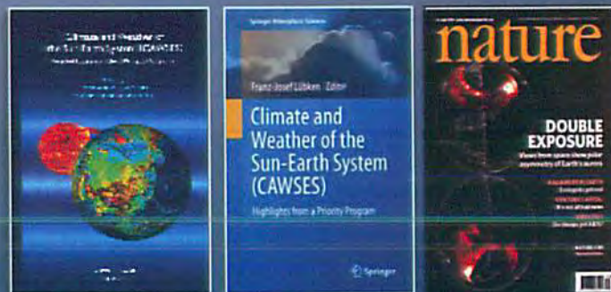
CAWSES I-2007 book; German CAWSES Priority Program; Conjugate imaging of aurora in both hemispheres and inter-hemispheric currents (Laundal and Østgaard, Nature, 2009)
